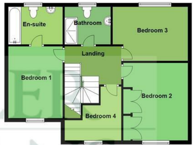
First Floor Approx. 715.4 sq. feet
